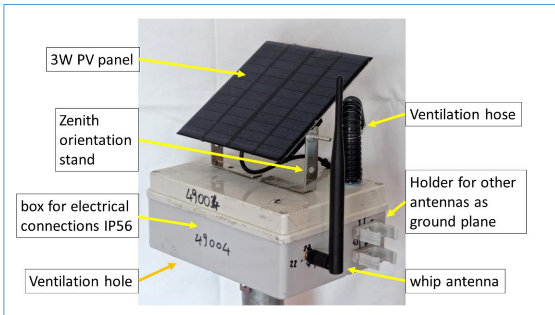
Figure 10 - A general purpose active case for TX node
