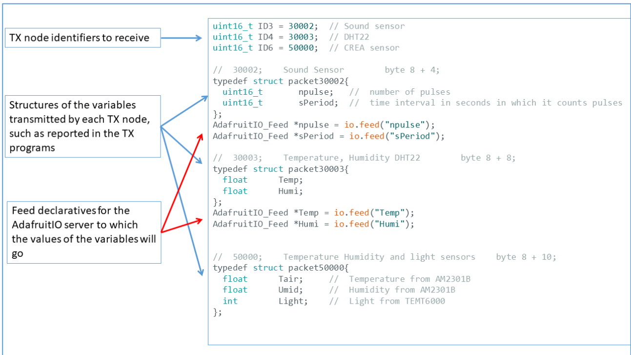
Figure 27 - Packet.h content, first part
