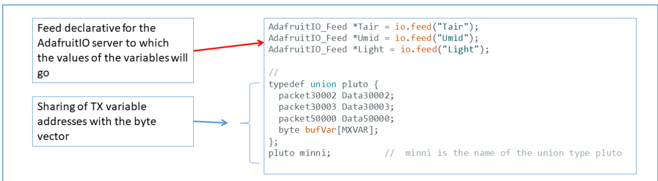
Figure 28 - Packet.h content, second part
