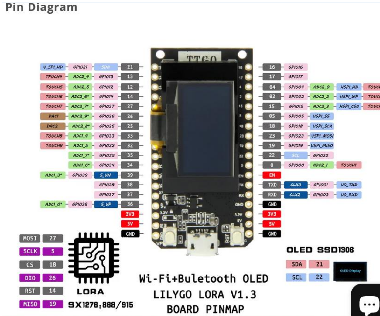
Figure 18 – LILYGO® TTGO LORA32 868/915Mhz (LoRa32 V1.3). Board Pinmap
