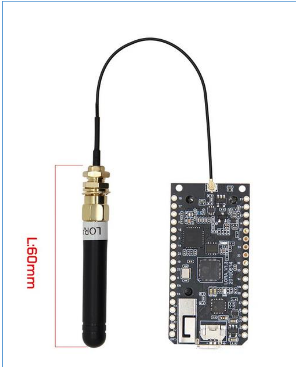
Figure 17 - LILYGO® TTGO LORA32 868/915Mhz (LoRa32 V1.3). This is an alternative board to version 1.0
