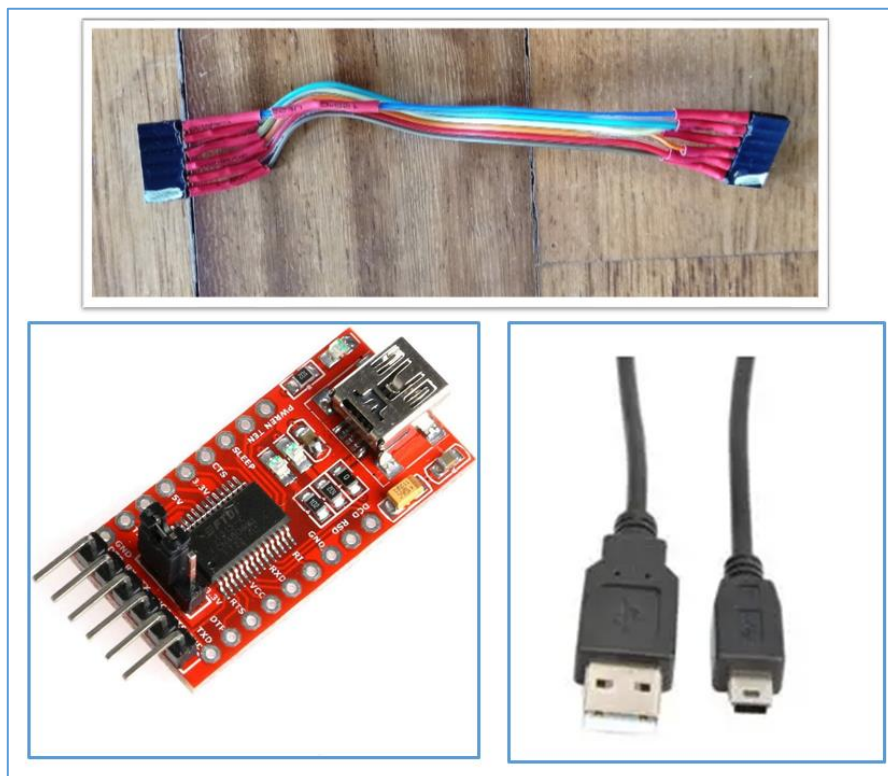
Figure 8 – Items needed for the connection between PC and the ProMiniLoRa board shown in Figure 6
