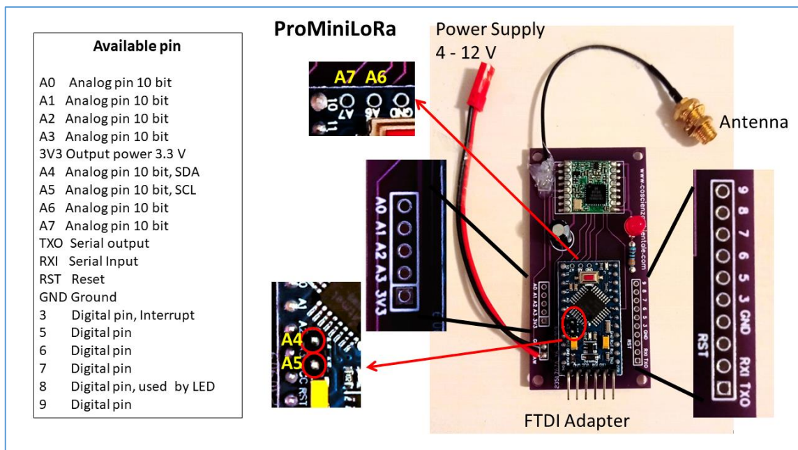
Figure 6 – ProMiniLoRa, the board I made
