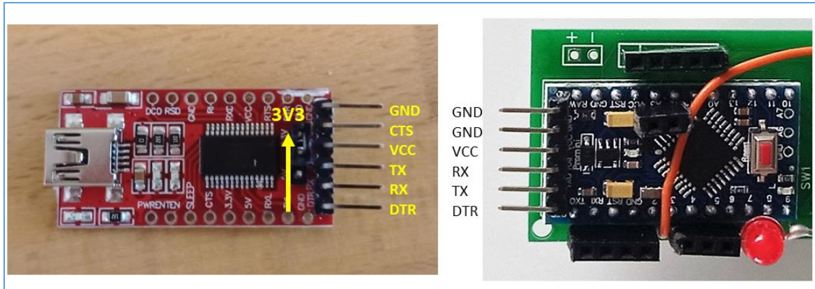
Figure 9 - Pins to be connected by means the cable shown in shown in
