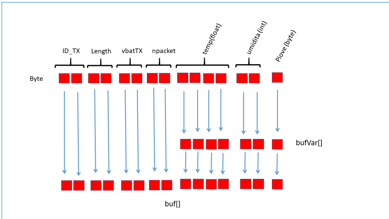
Figure 22 - Correspondence between the bytes of the variables and those of the arrays
