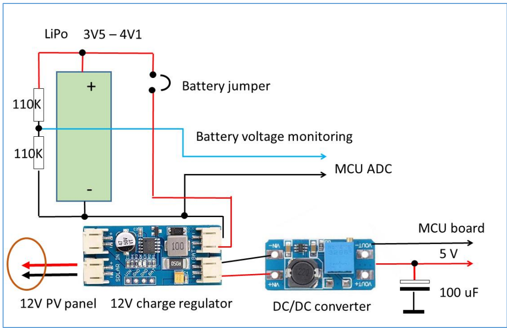
Figure 11 – Electronics inside the box for the solar power supply
