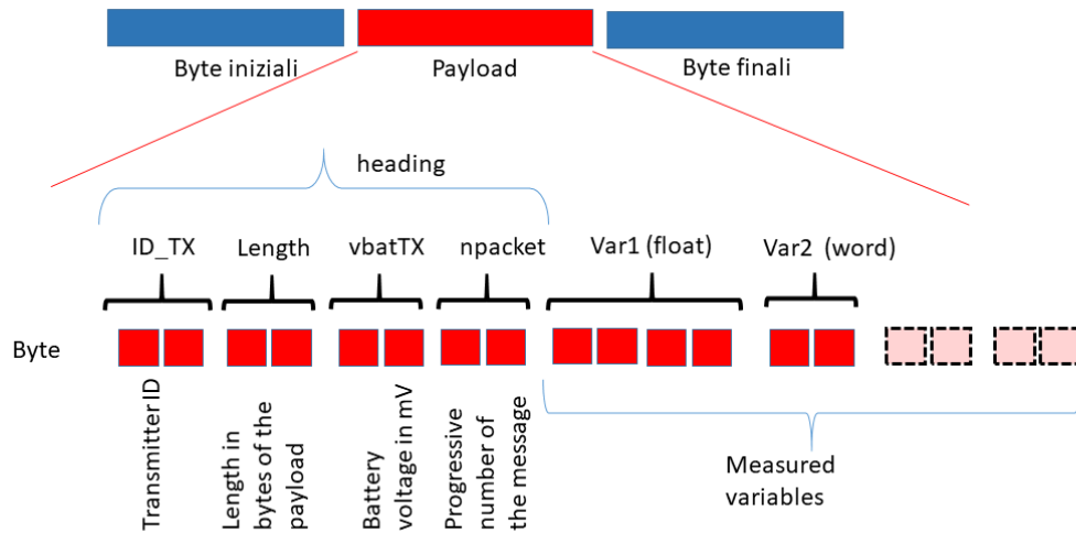
Figure 20 – Payload structure of a message for a MiniReteLoRa
