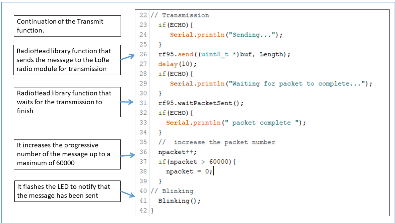
Figure 24– Transmit function, second part
