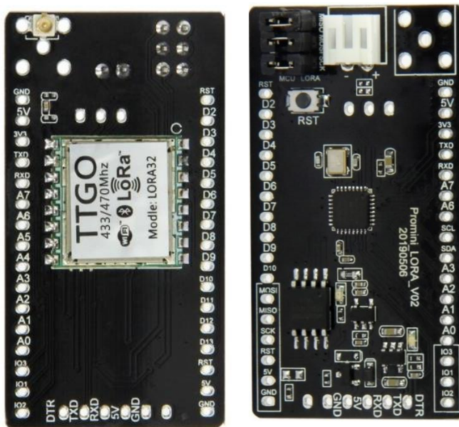
Figure 3 - The T-Deer board
