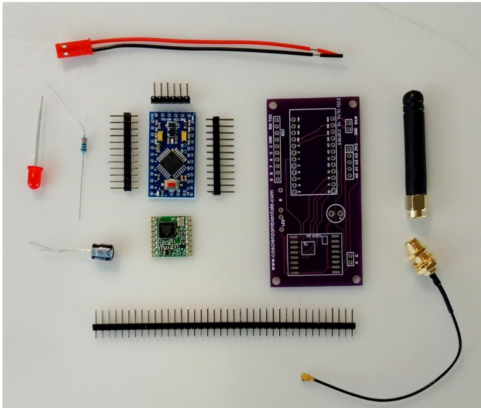
Figure 7 - Components of the ProMini LoRa board
