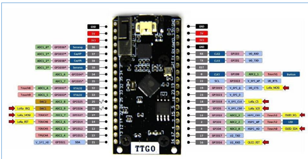
Figure 14 - The board LoRa32 V1.0 (errata: pin 19 = LoRa MISO, not MOSI)
